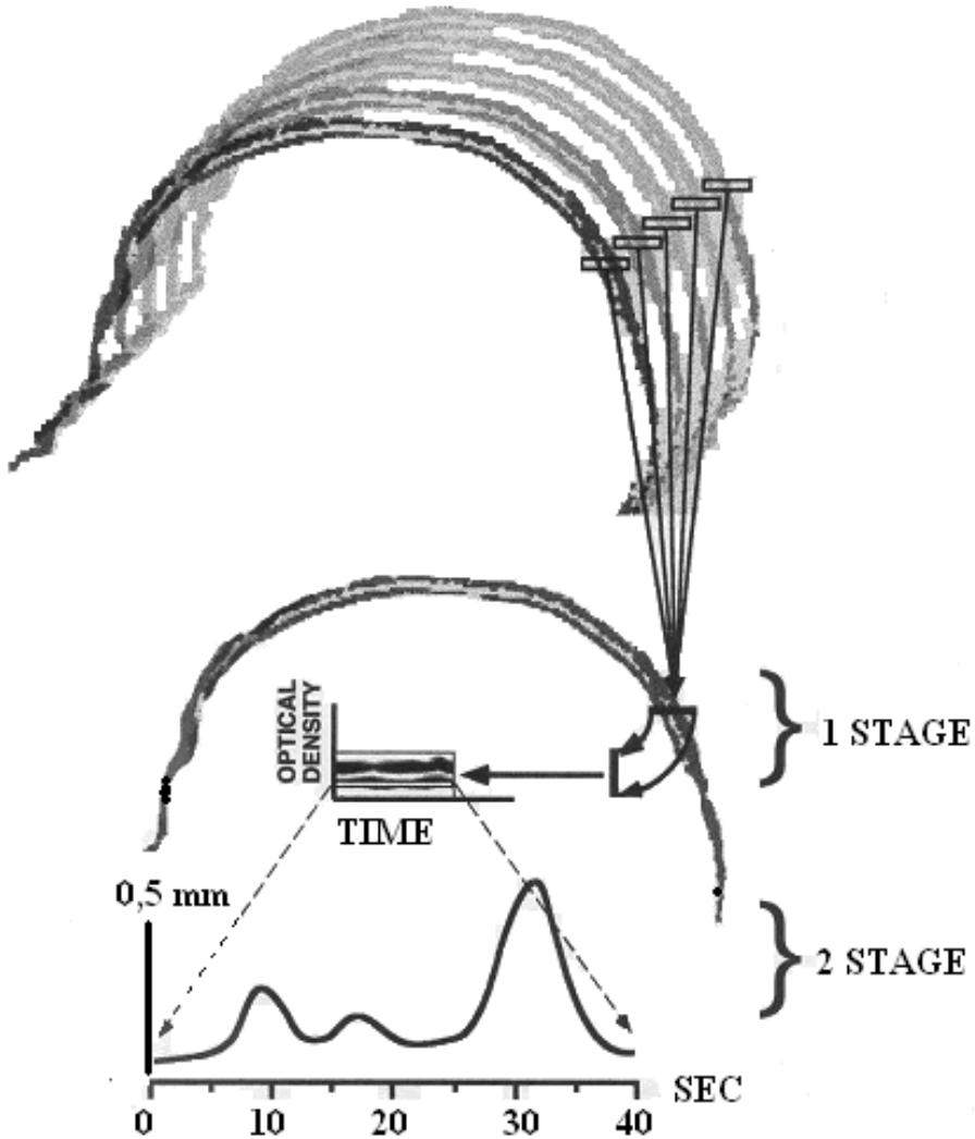
Figure 5. Principle of transforming individual regions of image series into the amplitude-time plot: (a) input of the image series into a computer and specification of the analyzed region; (b) collocation of images and creation of the intermediate image; and (c) transformation of the intermediate image into the amplitude-time plot.
