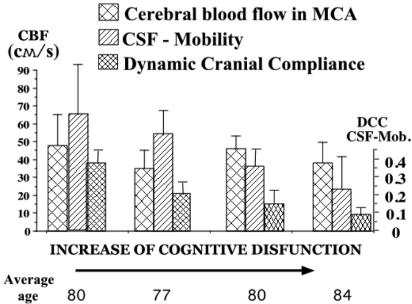
Figure 4. Dependence between value of DCC , Cerebral blood flow and CSF – mobility in aging human groups which are different by level of cognitive dysfunction.
