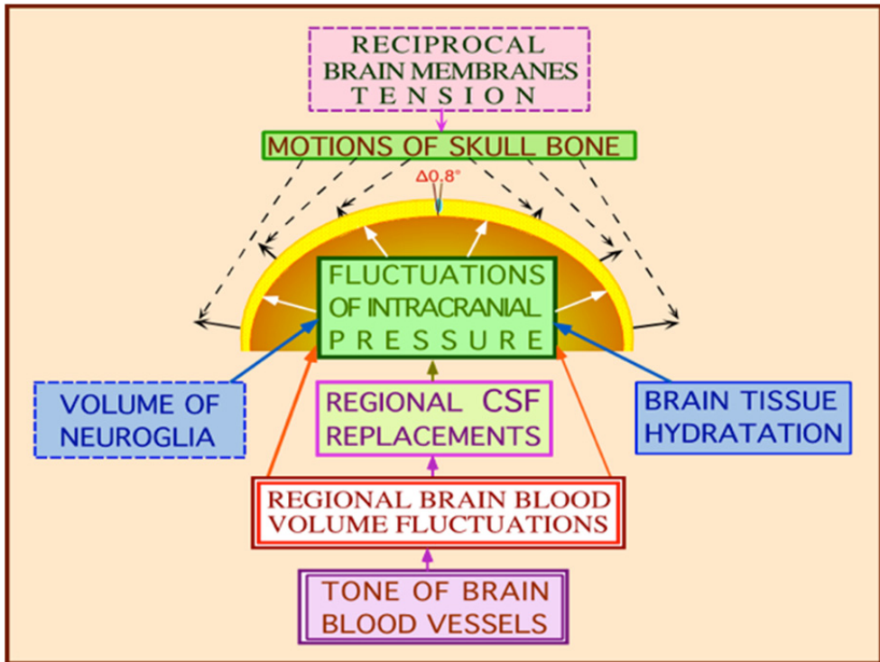
Figure 9. Schematic representation of skull move motion, initiated intracranial pressure , roun indicate physiological origin (BROW) but may be pathological origin – (BLUE).
